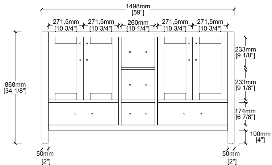
FRONT VIEW
